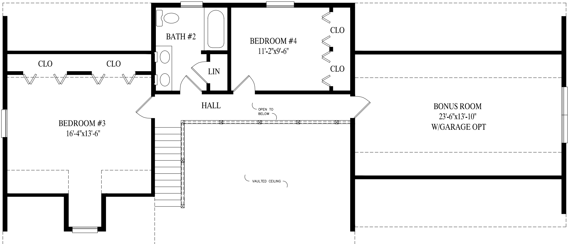
Proposed 2nd Floor - 645 sq. ft. w/ garage option - 995 sq. ft.
