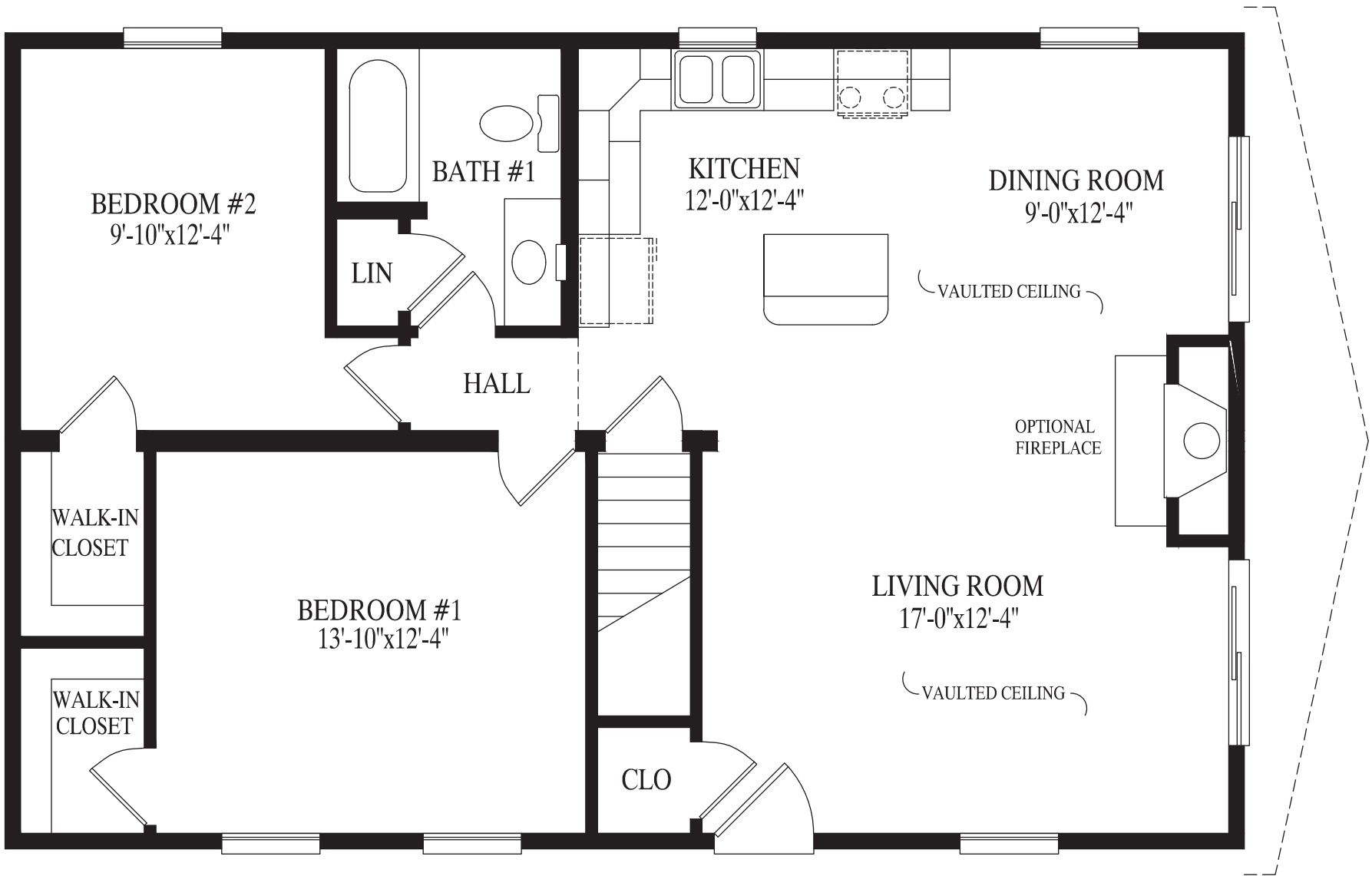
BRYCE 26'-4" X 40'-0" 1053 Sq. Ft.
